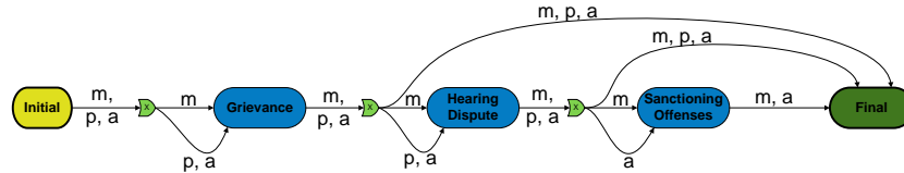
Fig. 5 Arbitration performative structure
