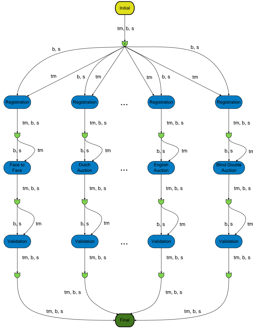
Fig. 3 TradingTable performative structure
