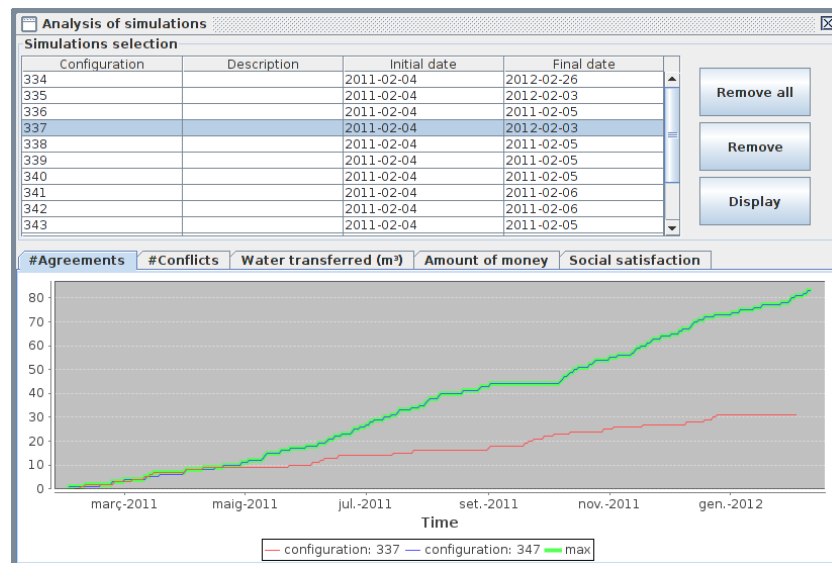
Fig. 9 Analysis of different configurations. Thick line represents the optimal solution, in this case the max number of agreements
