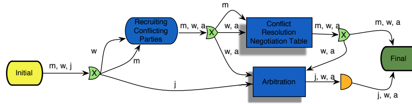
Fig. 4 Grievances performative structure
