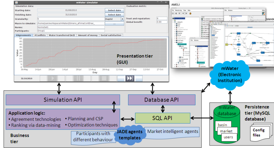
Fig. 6 Multi-tier architecture of the mWater system
