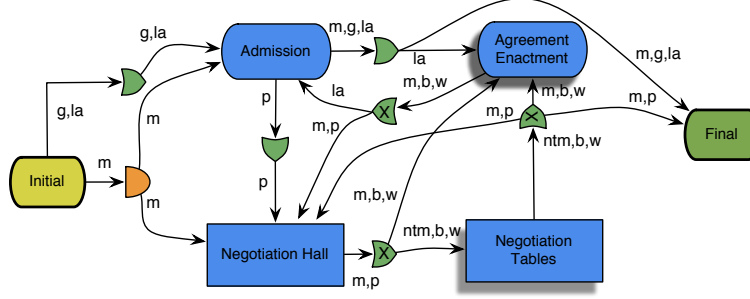
Fig. 7 Performative structure of a generic electronic institution for negotiation. Roles: g - Guest; p - Participant; b - Black; w - White; m - Mediator; ntm - Negotiation Table Manager; la - Legal Authority.
