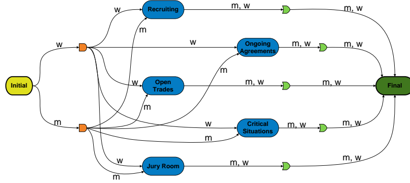
Fig. 2 TradingHall performative structure
