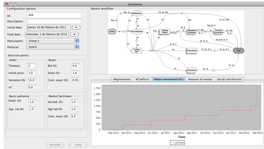
Fig. 8 The mWater simulator in action
